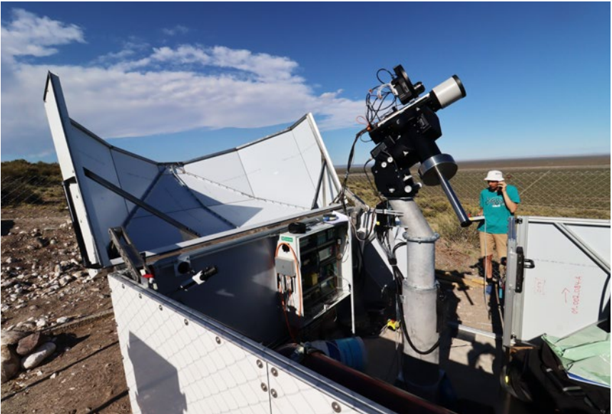
► AUGER-CZ – Telescope FRAM used to monitor atmospheric conditions at Pierre Auger Observatory in Argentina which detects the highest energy cosmic rays coming from the Universe
